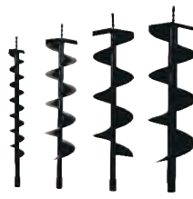
EARTH AUGER BIT A TYPE (60MM TO 300MM)
